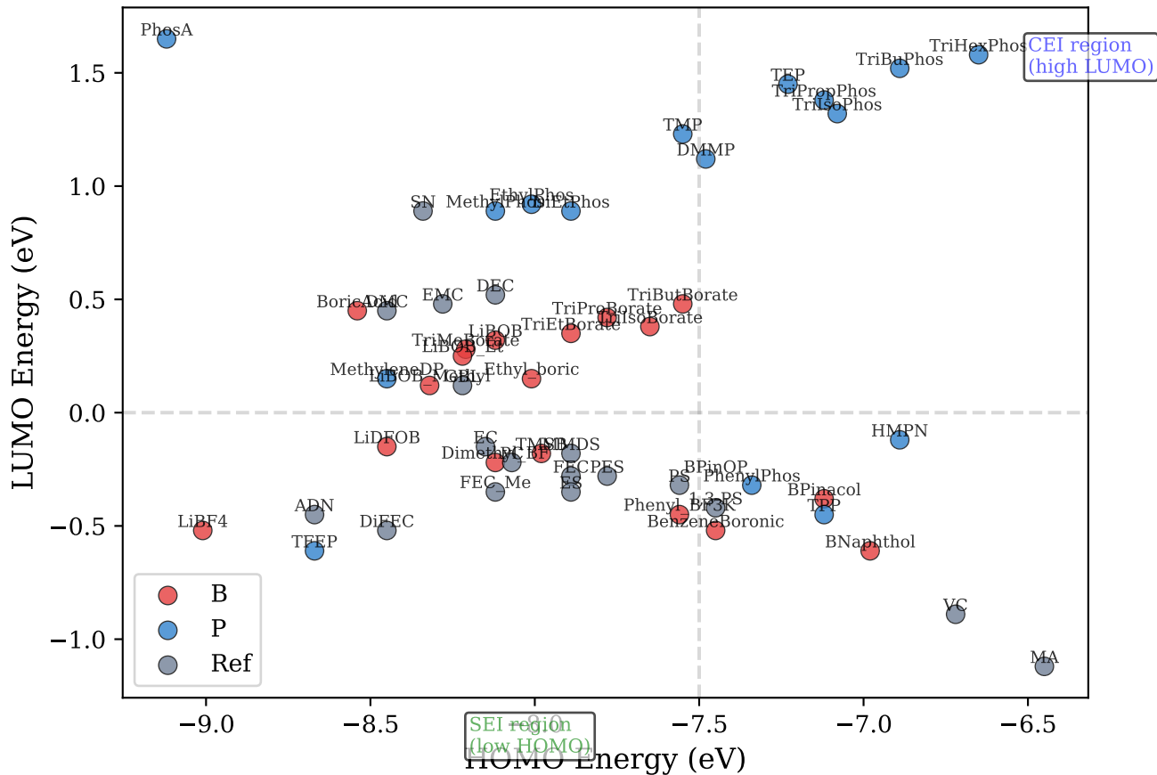
Frontier Orbital Energies of 64 Known Additives
