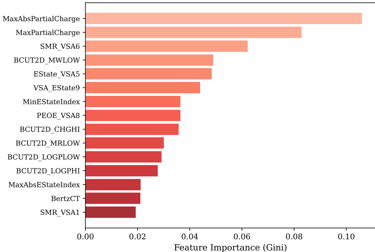
Top 15 Most Important Molecular Descriptors (Random Forest)
