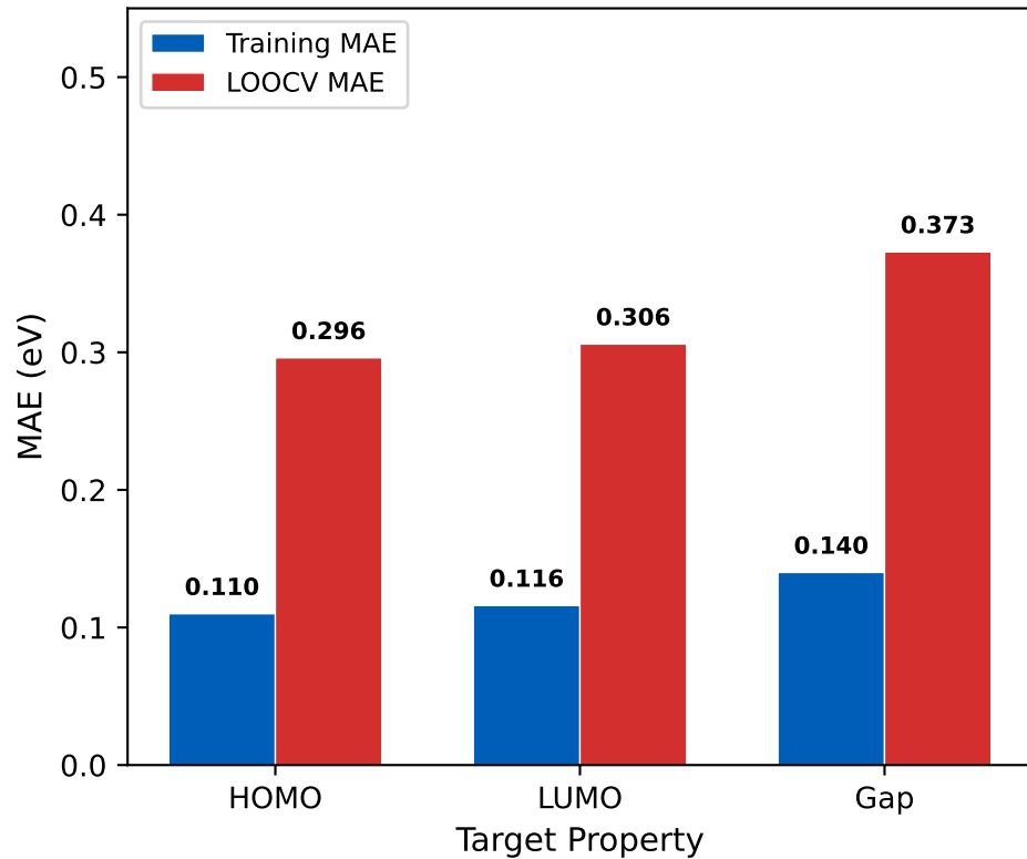
Prediction Error: Training vs LOOCV
