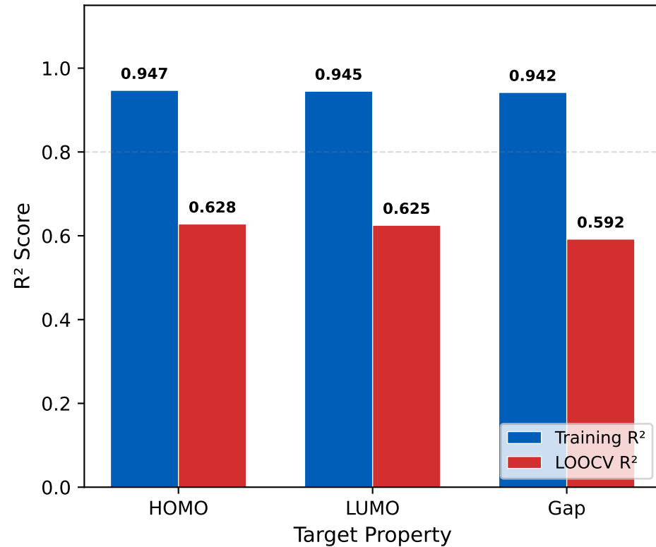
Model Performance: Training vs LOOCV
