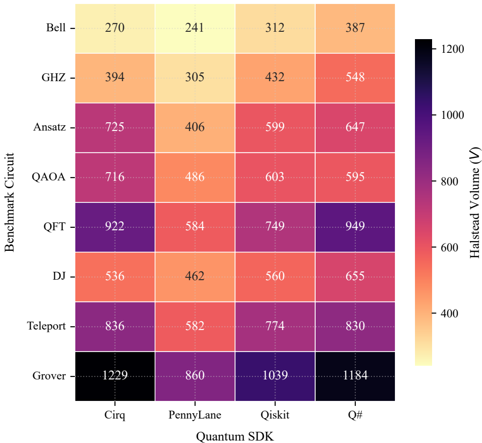
Mean Halstead Volume ( V ) by Circuit and SDK (averaged across both import conditions)
