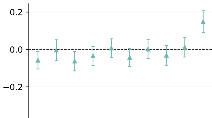
Text similarity
