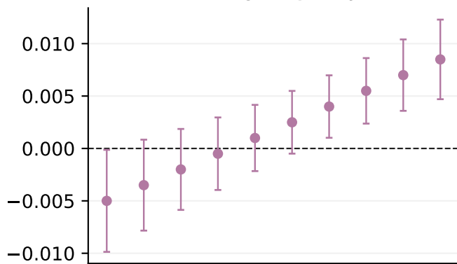
Lexical complexity
