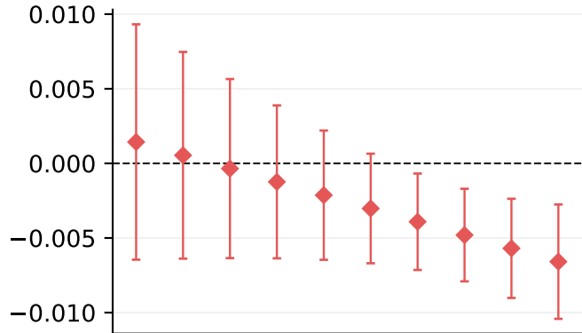
Grade
