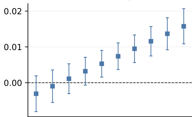
Syntactic complexity
