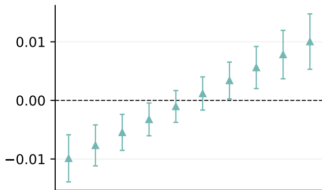
Text similarity
