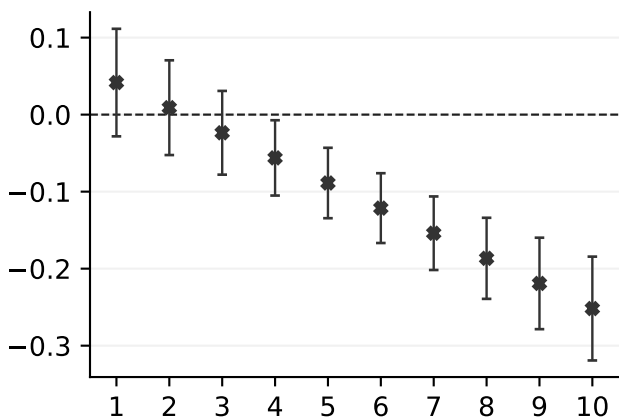
Grade
