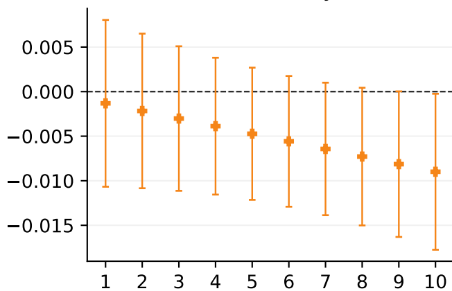
Text similarity
