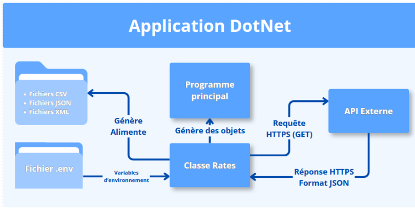
Figure 5: Architecture de l'application console
