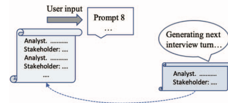
Figure 10: Iterative generation approach for structured elicitation artifacts by Görer and Aydemir [18]
