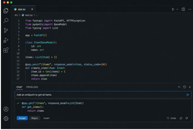
Figure 11: An example of an inline chat interface integrated into a code editor, allowing developers to interact with an LLM for real-time code suggestions and debugging assistance.
