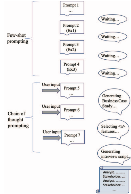
Figure 9: Batch generation approach for structured elicitation artifacts by Görer and Aydemir [18]
