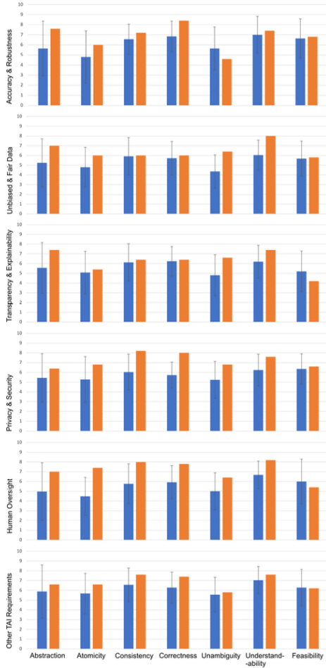
Figure 8: Comparative analysis of requirements quality attributes for ChatGPT-generated and human-generated requirements by Ronanki et al. [34]
