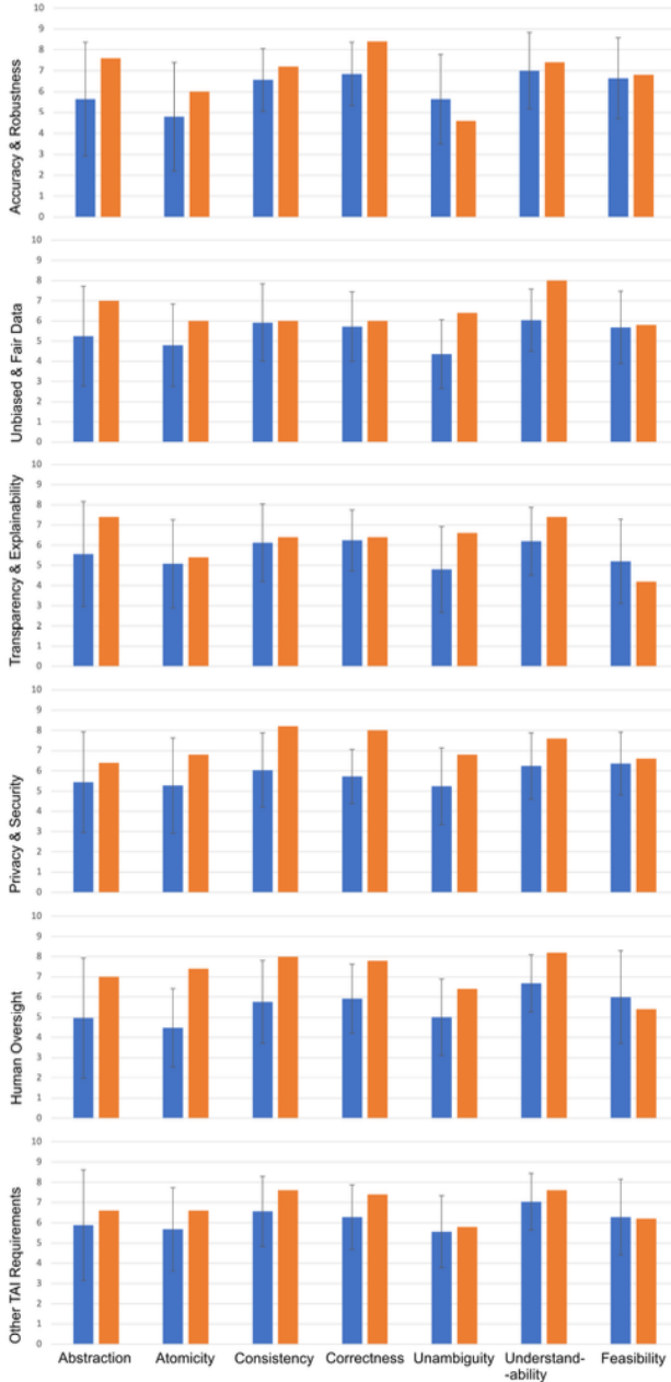
Figure 8: Comparative analysis of requirements quality attributes for ChatGPT-generated and human-generated requirements by Ronanki et al. [29]
