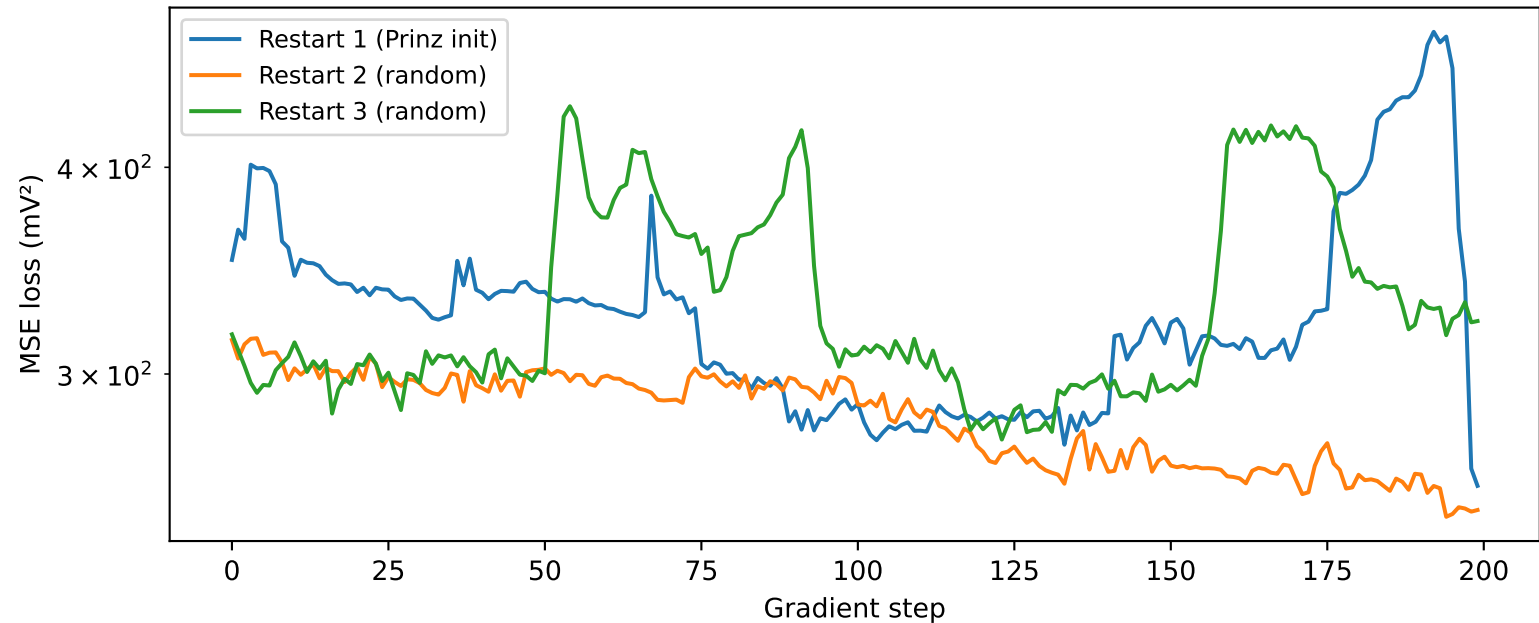
Gradient descent learning curves (3 restarts)
