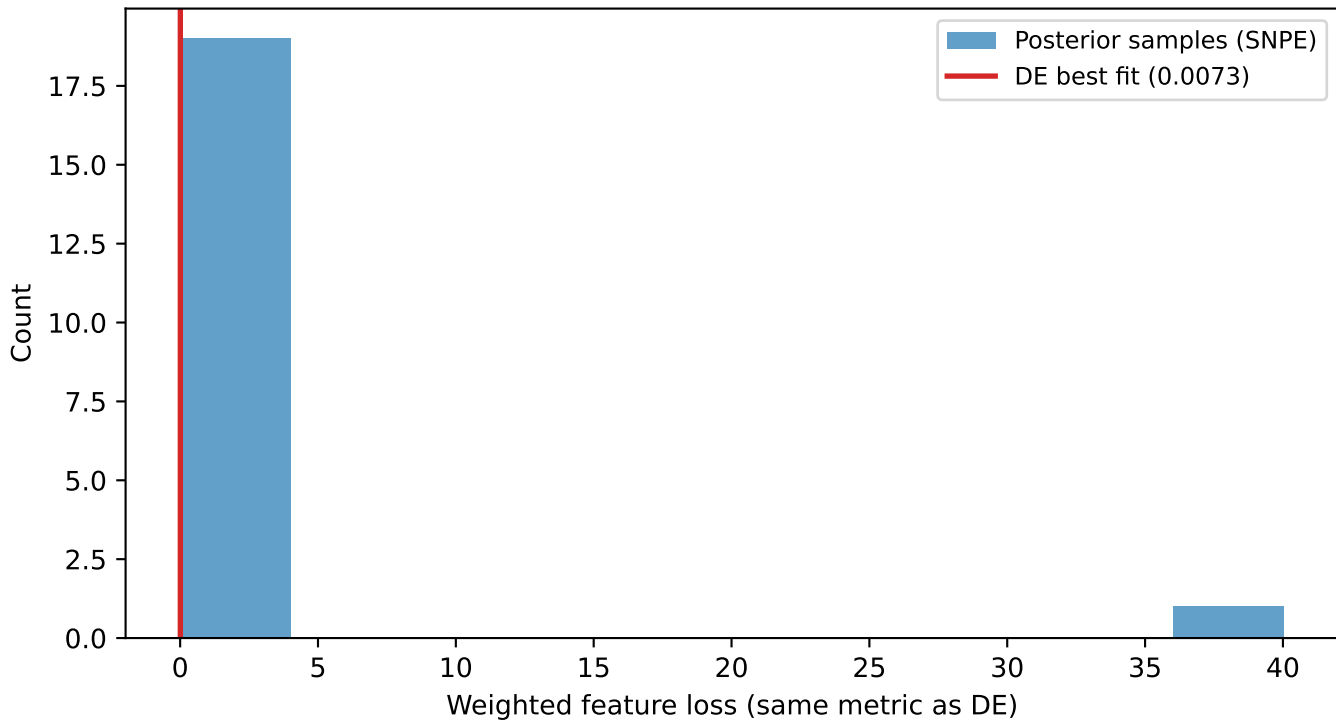
Posterior samples vs. DE: same-metric loss comparison
