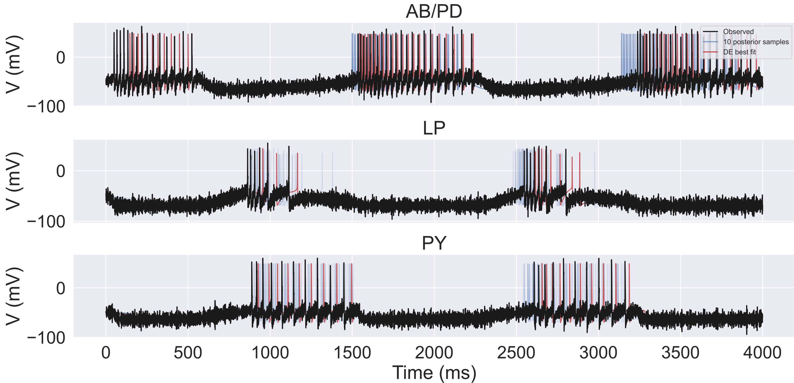
Degeneracy: multiple parameter sets reproduce the observed rhythm
