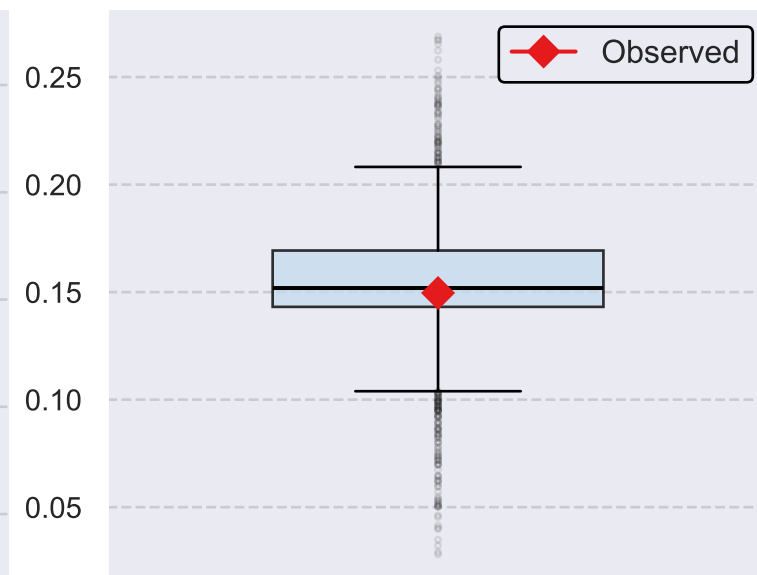
PY phase
