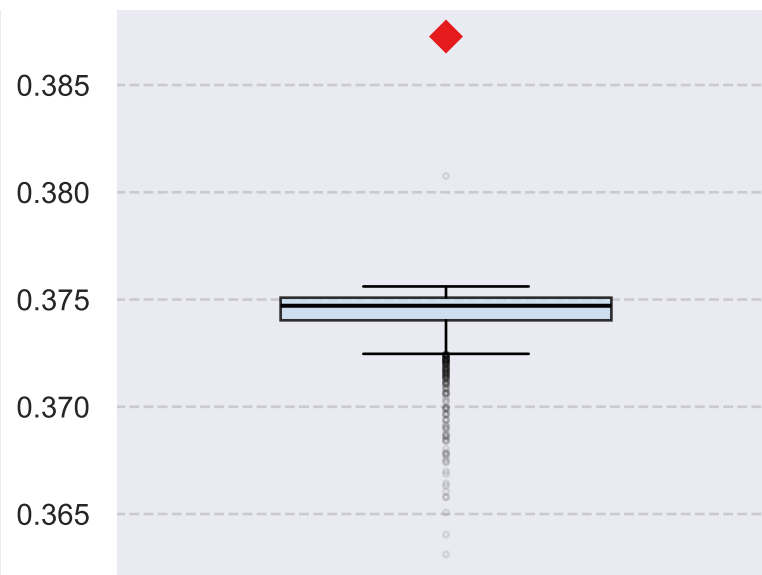
LP phase
