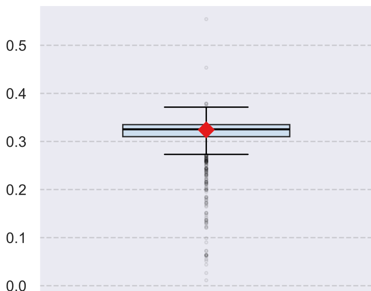
AB/PD spikes/burst
