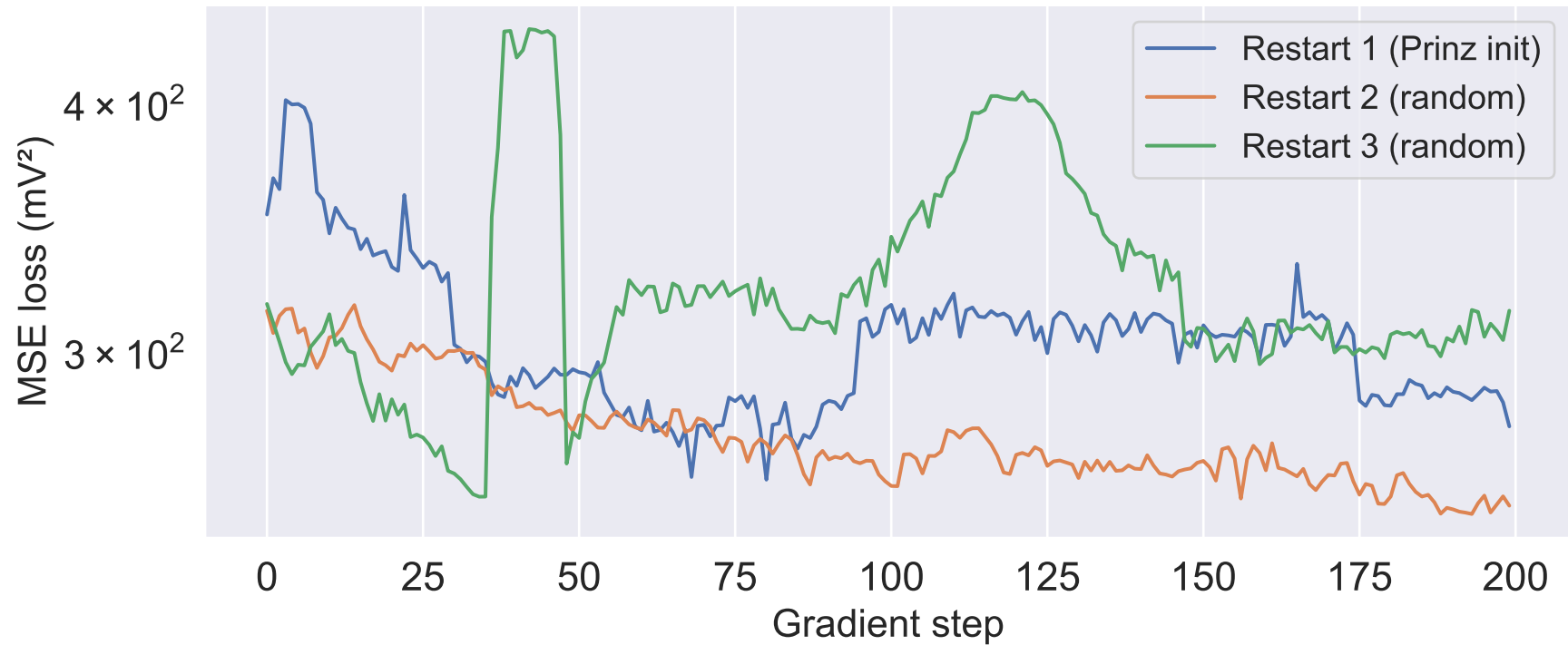
Gradient descent learning curves (3 restarts)
