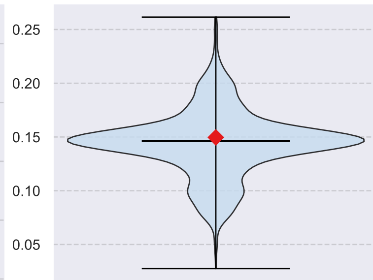
PY phase
