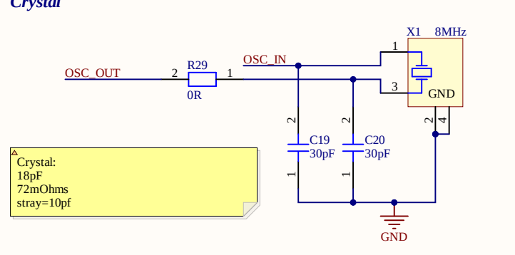
U_Interface_STM32 Interface_STM32.SchDoc
