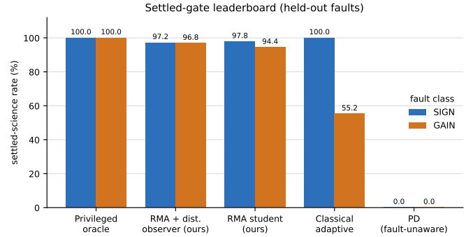
Fig. 1. Headline standings on the two controllable continuous fault classes, ordered best to worst by combined settled-science rate. The settled gate spreads the controllers across the full range. The fault-unaware PD settles neither class, the classical adaptive law recovers SIGN but degrades on GAIN, and the RMA student approaches the privileged oracle on both. Every value is read from the same committed evidence as Table II.
