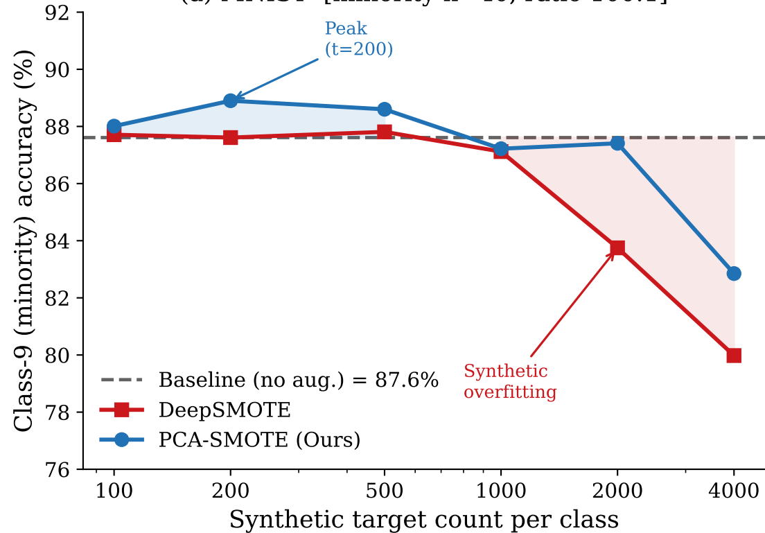
(a) MNIST [minority n=40, ratio 100:1]
