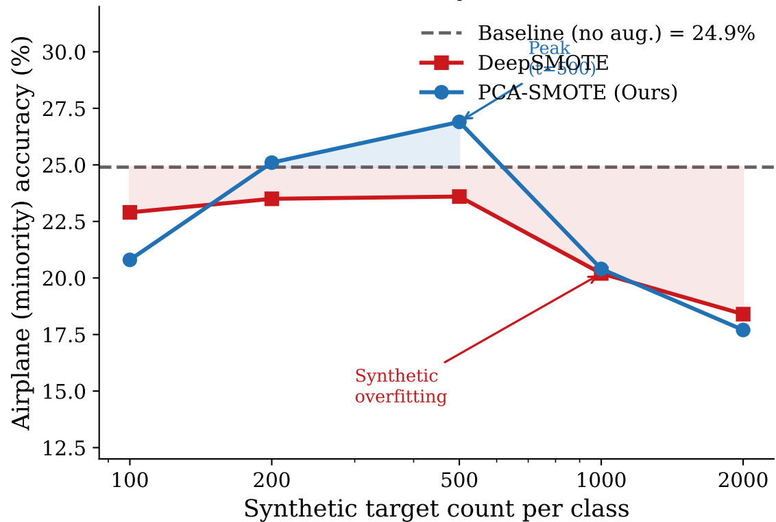
(b) CIFAR-10 [minority n=80, ratio 25:1]
