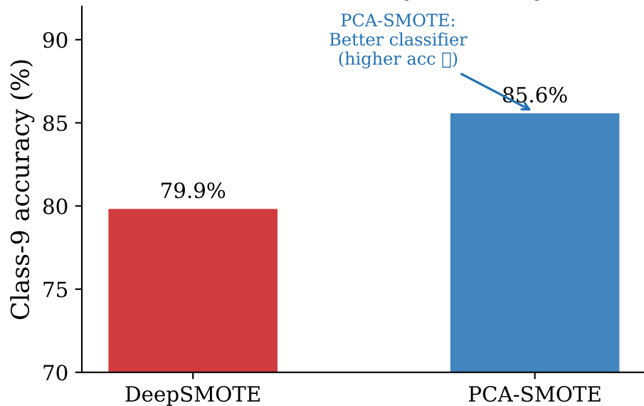
(b) Classifier Utility (accuracy)
