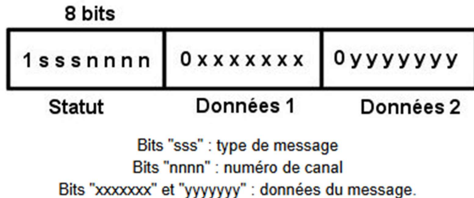
Figure 25 Trame MIDI
