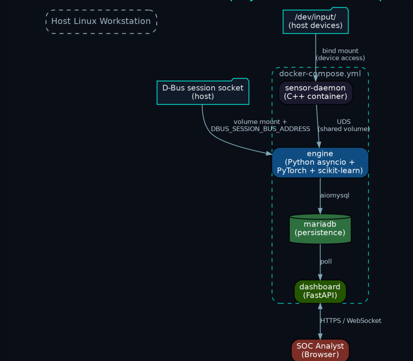
Figure 4.4: Docker Compose deployment showing host device/socket mounts into the containerized services.
