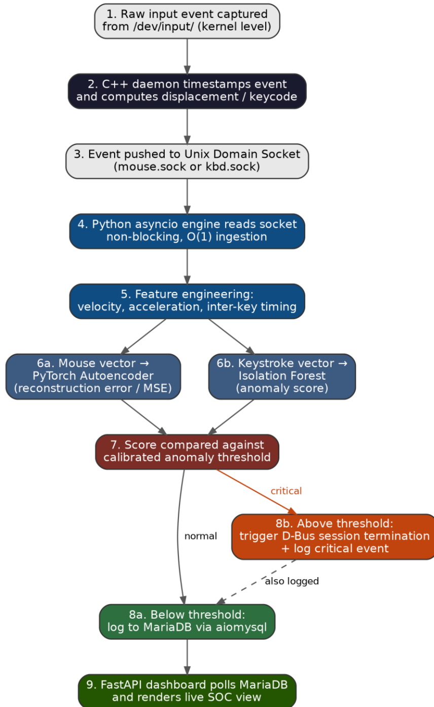
Figure 4.2: End-to-end data flow for a single telemetry event, from kernel capture to mitigation and dashboard rendering.
