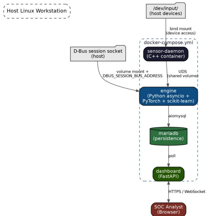
Figure 4.4: Docker Compose deployment showing host device/socket mounts into the containerized services.
