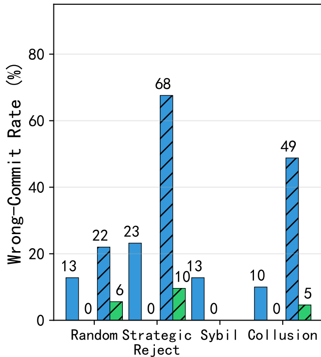
(b) Wrong commits: within vs below boundary
