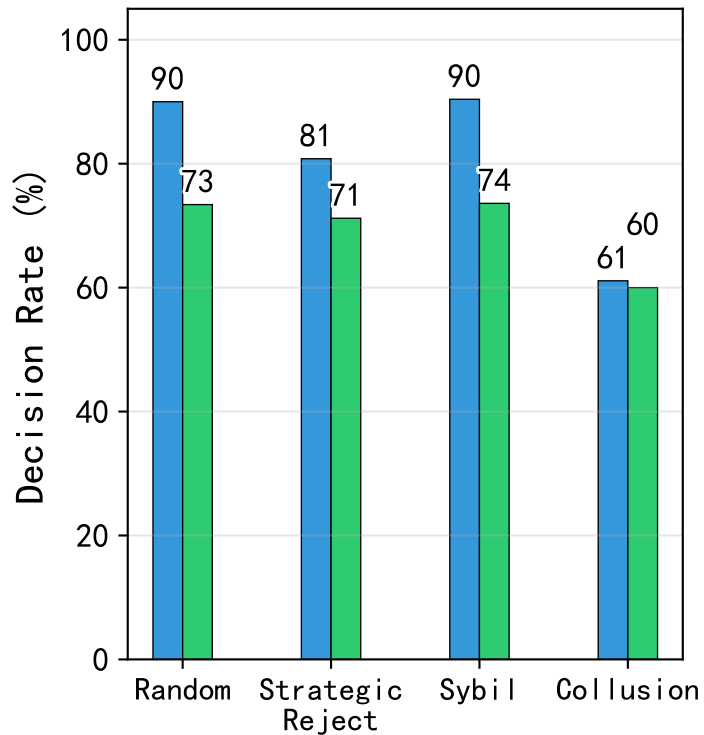
(a) Decision rate within boundary
