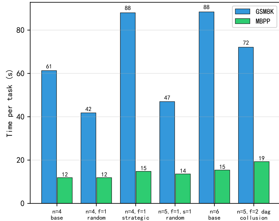
End-to-End Time per Task
