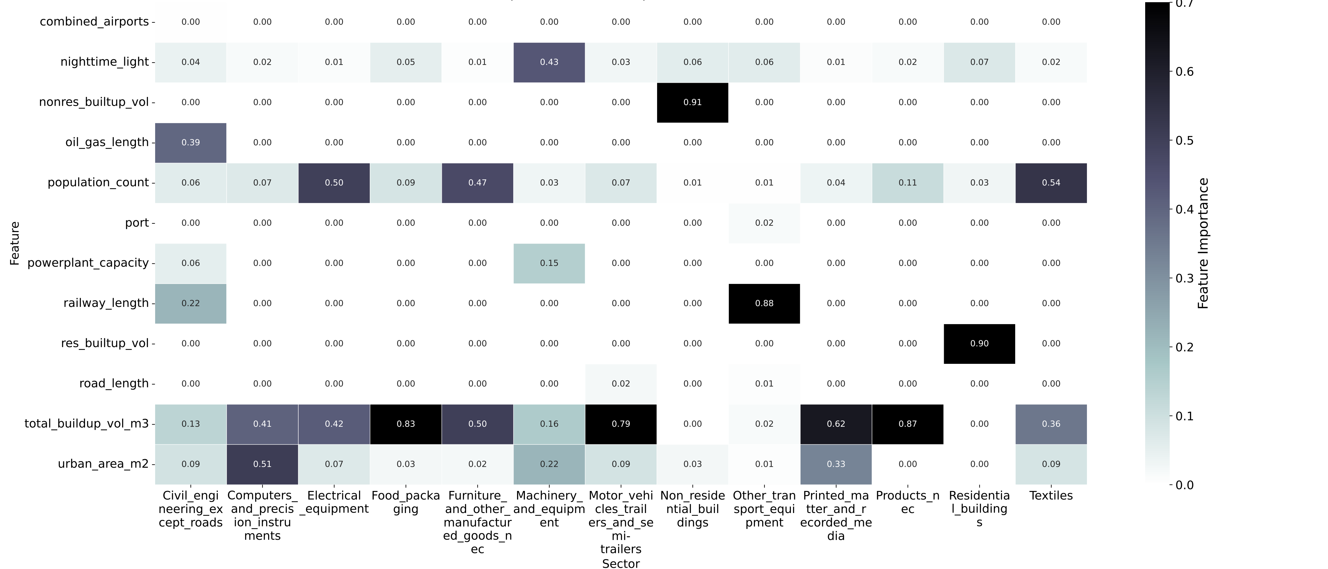
Feature Importance Heatmap for Income Class: LM
