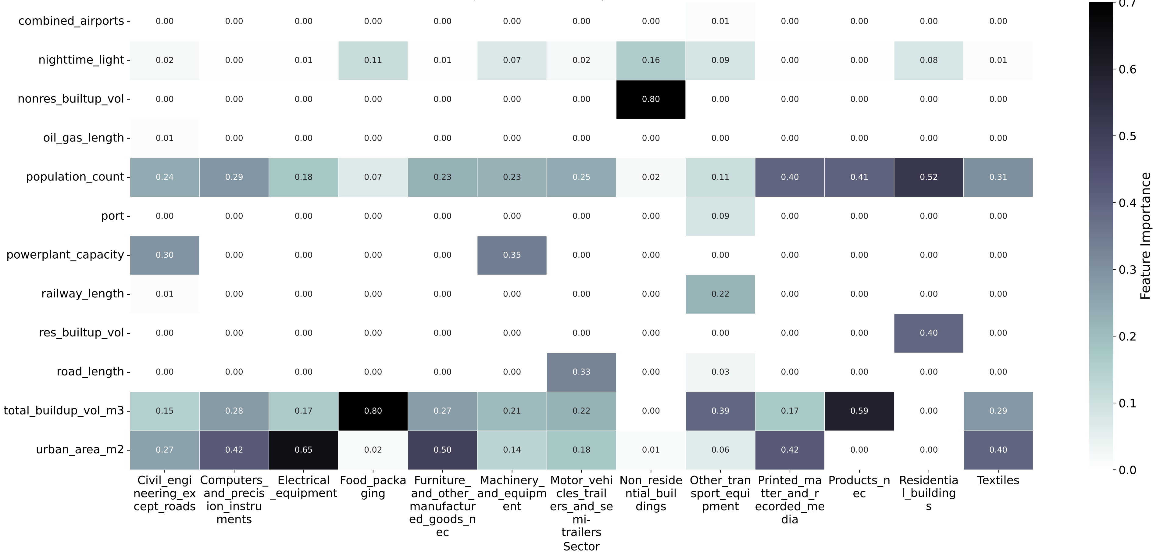
Feature Importance Heatmap for Income Class: UM
