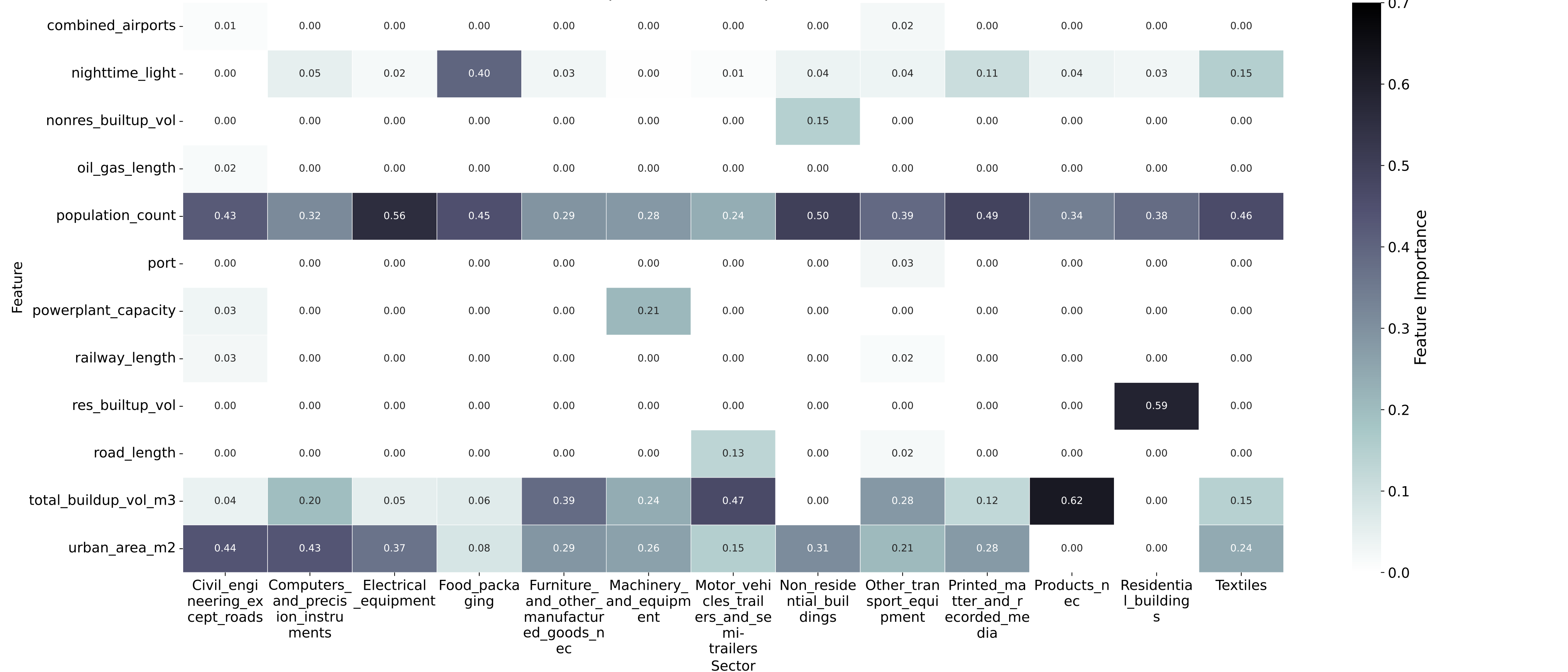
Feature Importance Heatmap for Income Class: H
