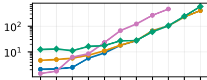
TRSV
