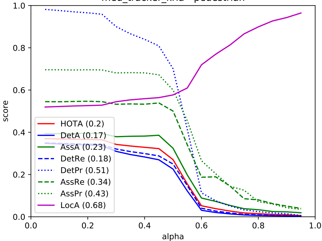
meu_tracker_kria - pedestrian
