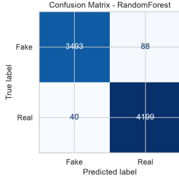
(c) Random Forest Confusion Matrix
