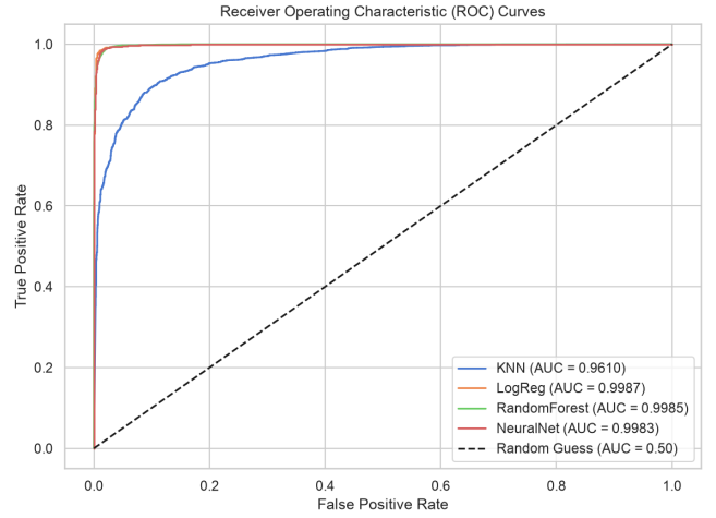
Fig. 4. ROC curves and Area Under the Curve (AUC) scores comparing KNN, Logistic Regression, Random Forest, and MLP Neural Network on the test set.
