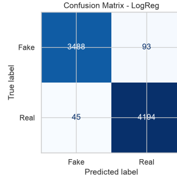
(b) Logistic Regression Confusion Matrix
