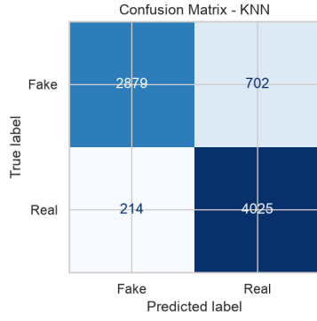
(a) KNN Confusion Matrix
