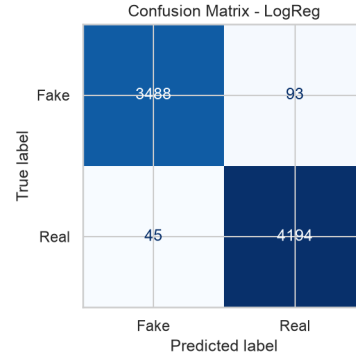
(b) Logistic Regression Confusion Matrix
