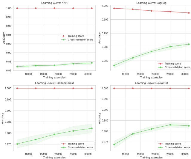
Fig. 3. Learning curves for the four classifiers showing training and validation accuracies over different training sizes.
