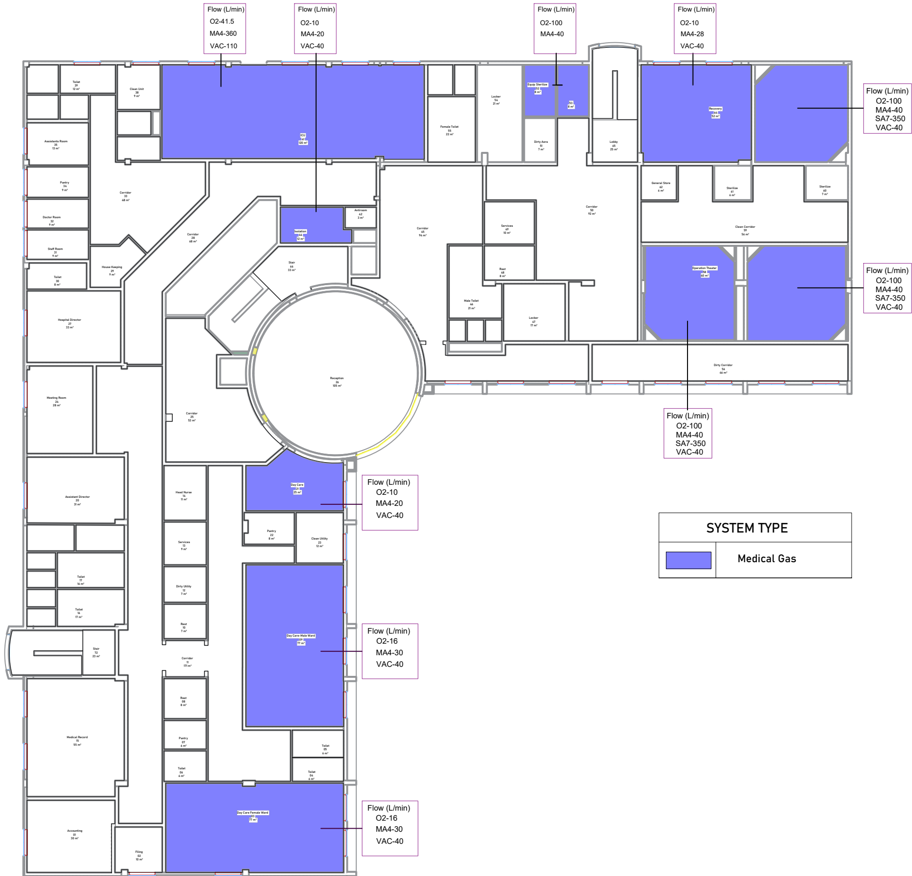
Ground Floor Plan - Medical Gas System
