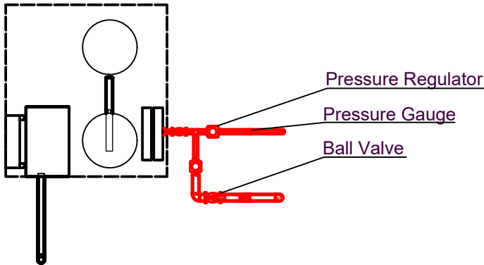
Compressor
