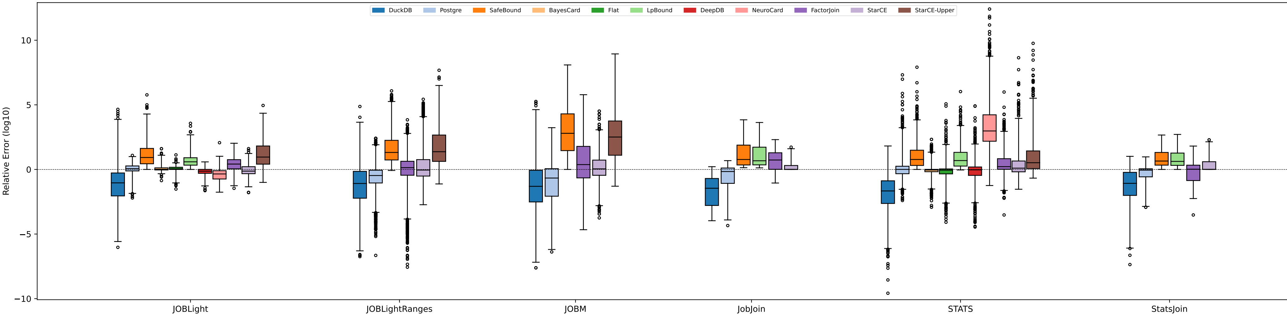
Q-Error (Boxplot by Benchmark)
