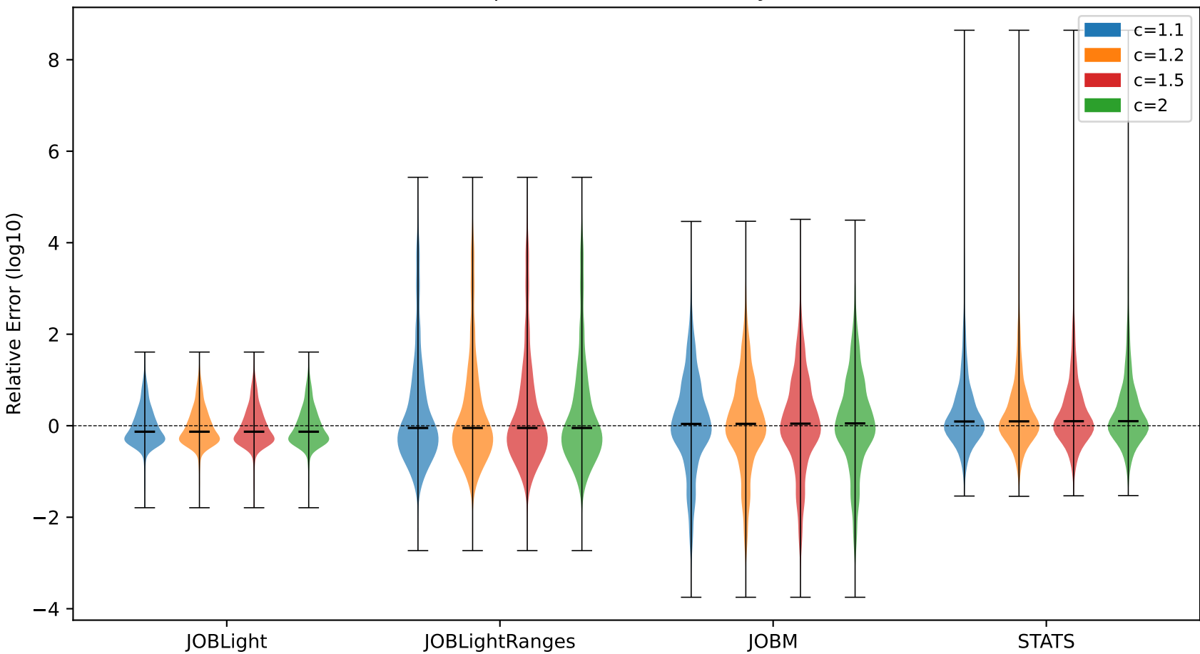
StarCE CompressPrecision (Violin by Benchmark)
