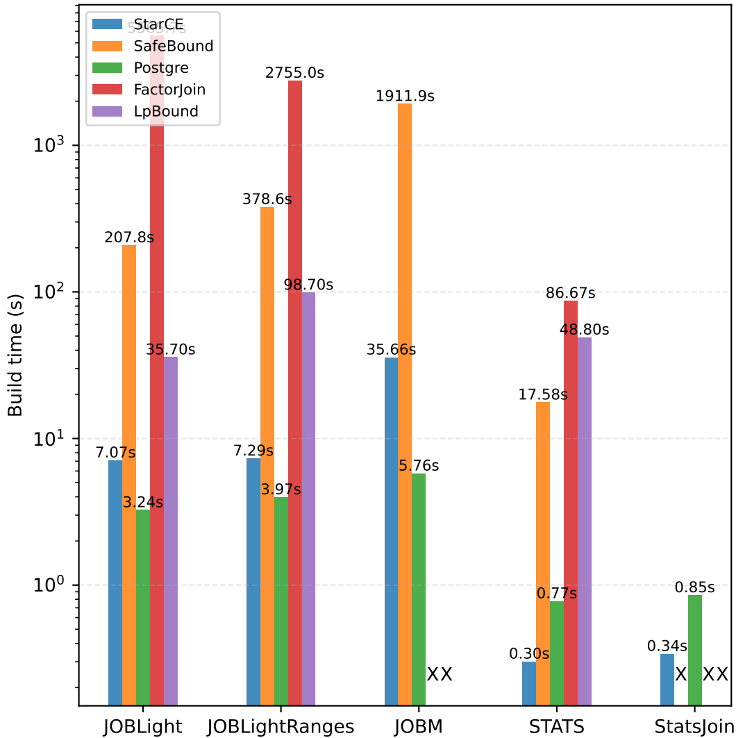
Build Time by Benchmark
