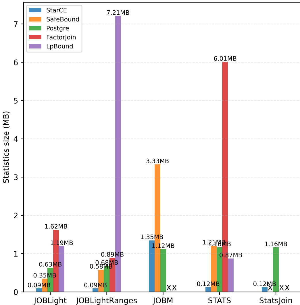
Statistics Size by Benchmark
