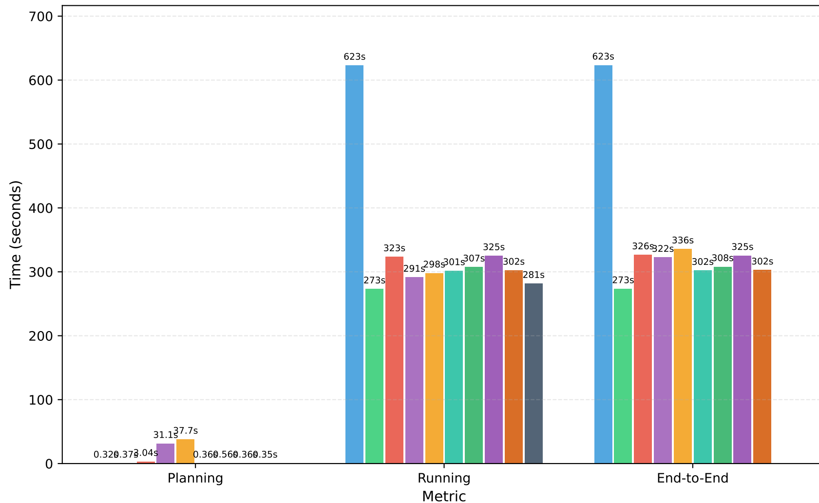
JOBLight
