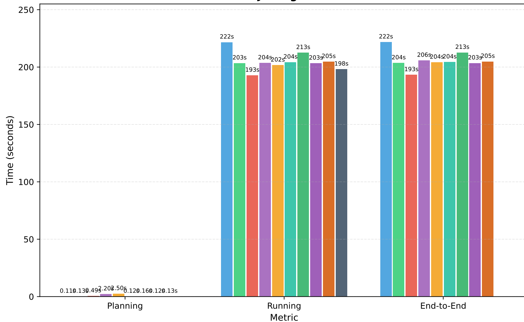
JOBLight
