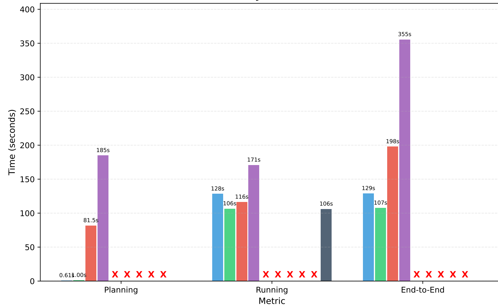
JOBLightRanges
