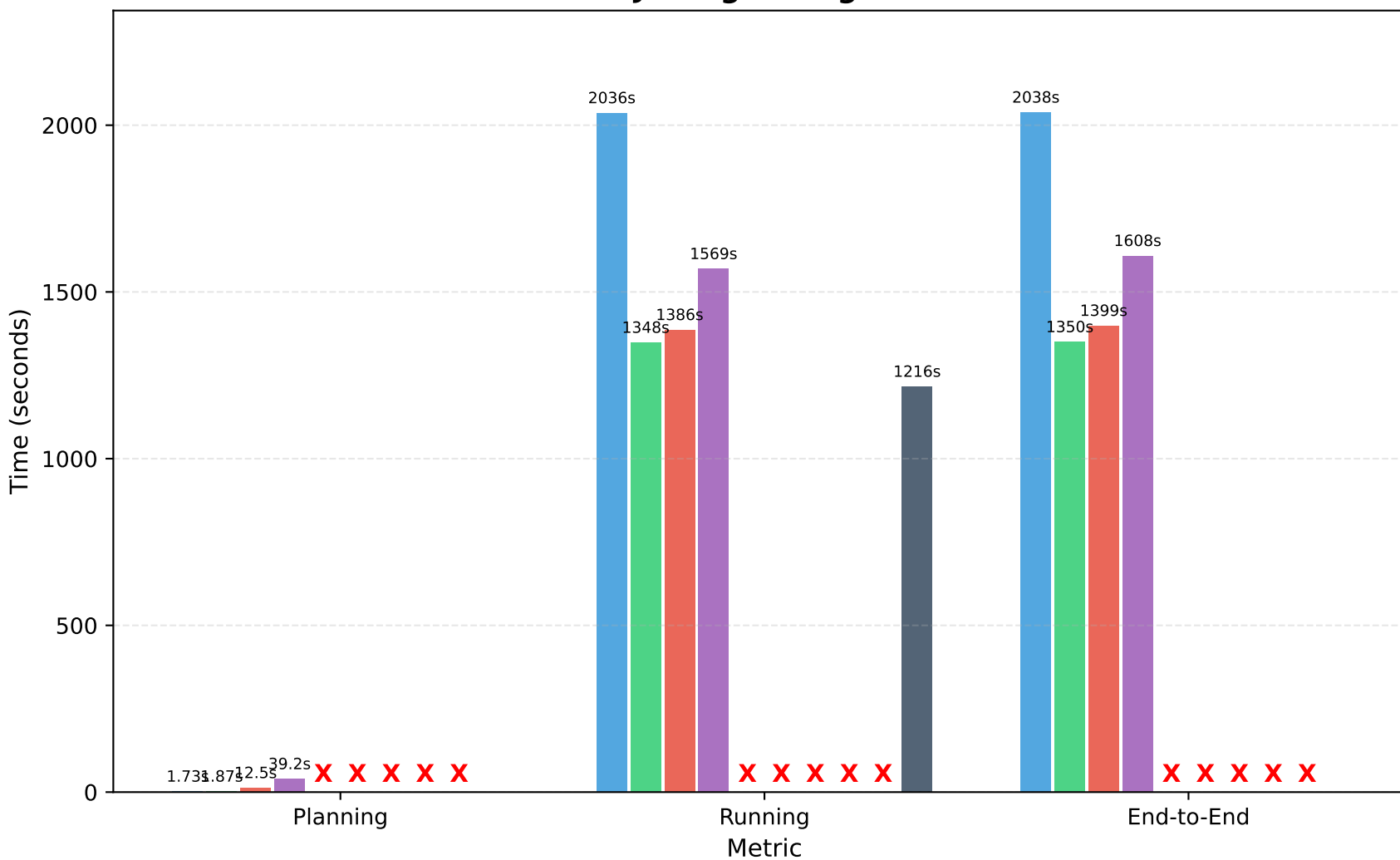
JOBLightRanges
