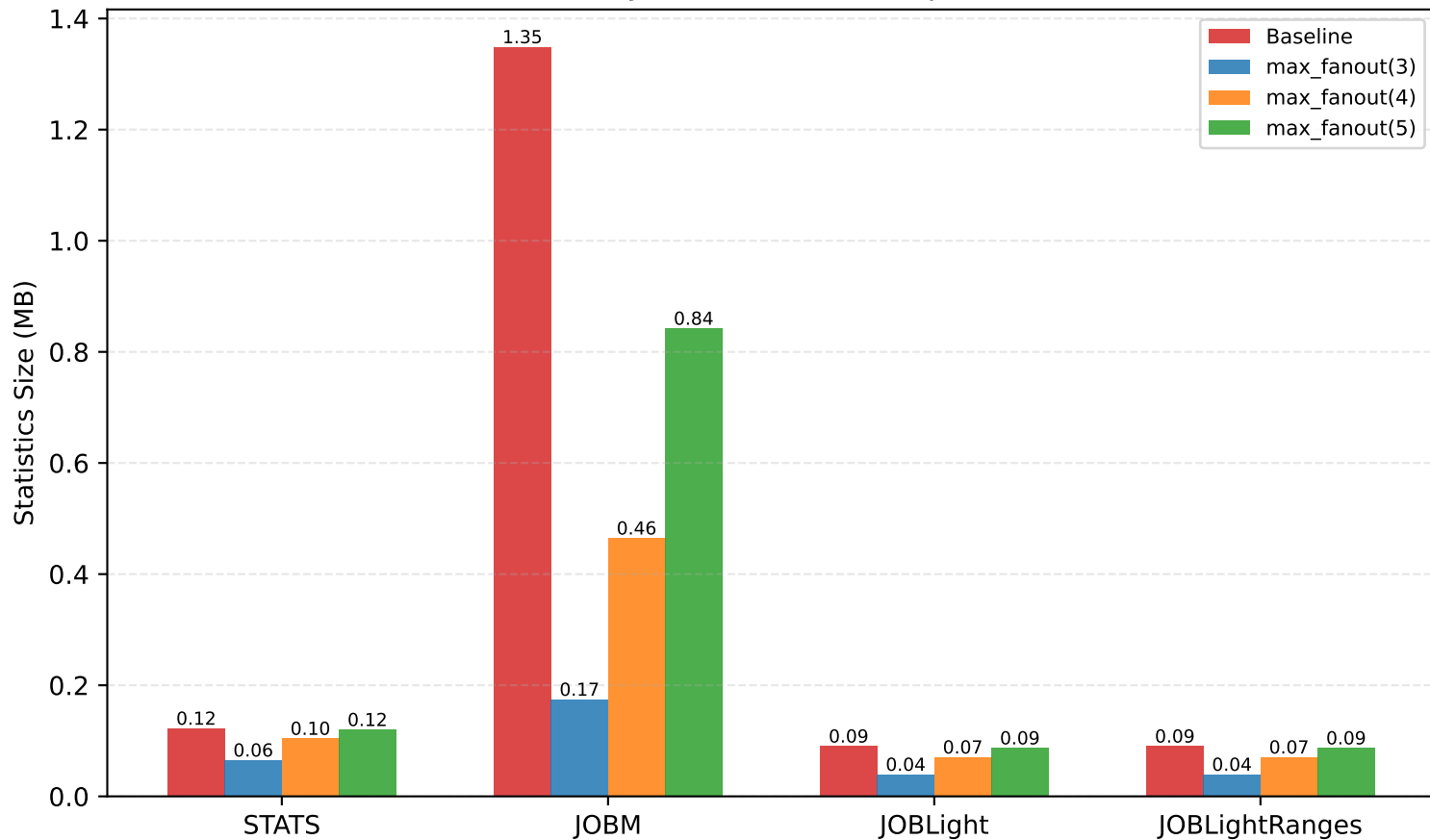
Statistics Size by Benchmark and SplitStar Variant
