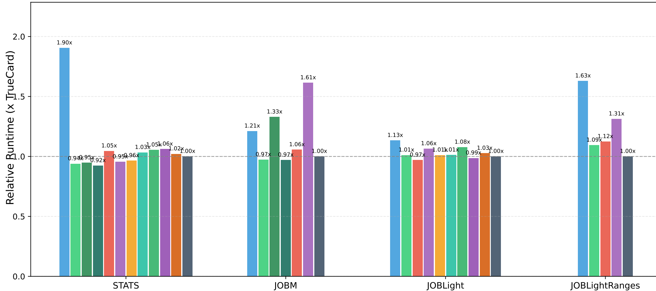
DuckDB (baseline: TrueCard DB)
