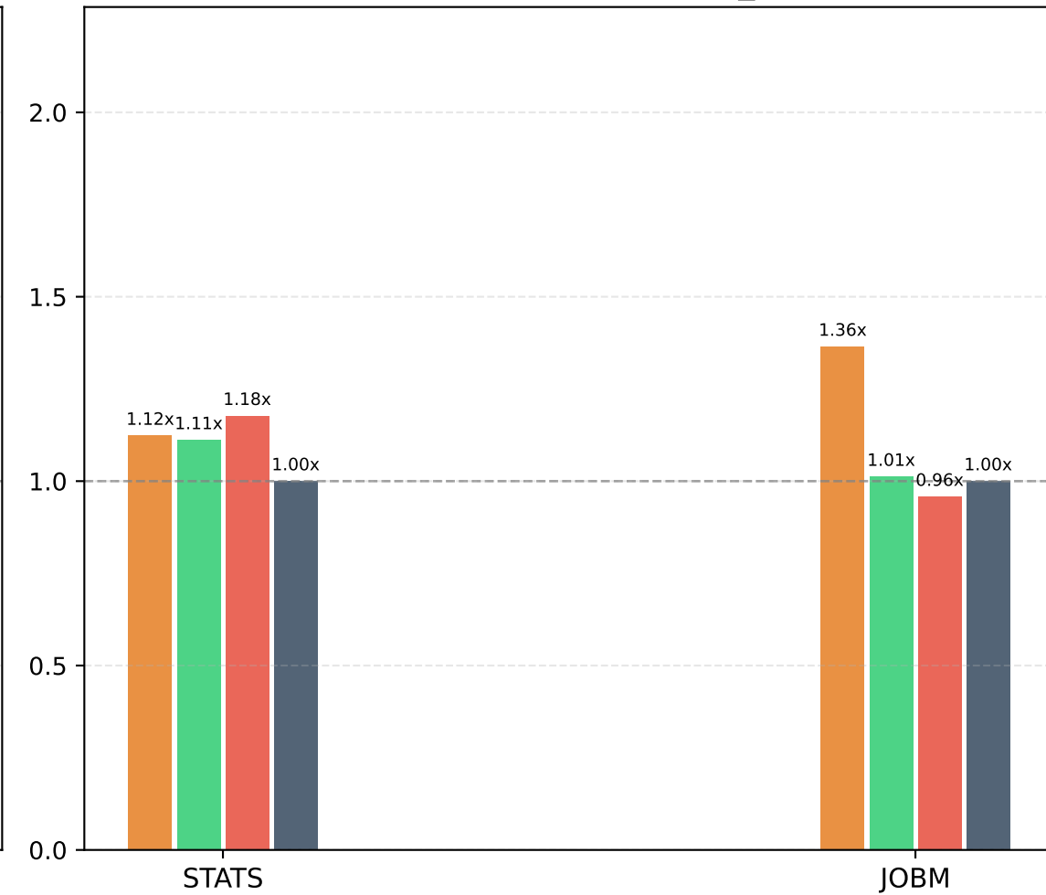
PostgreSQL (baseline: true_card PG)
