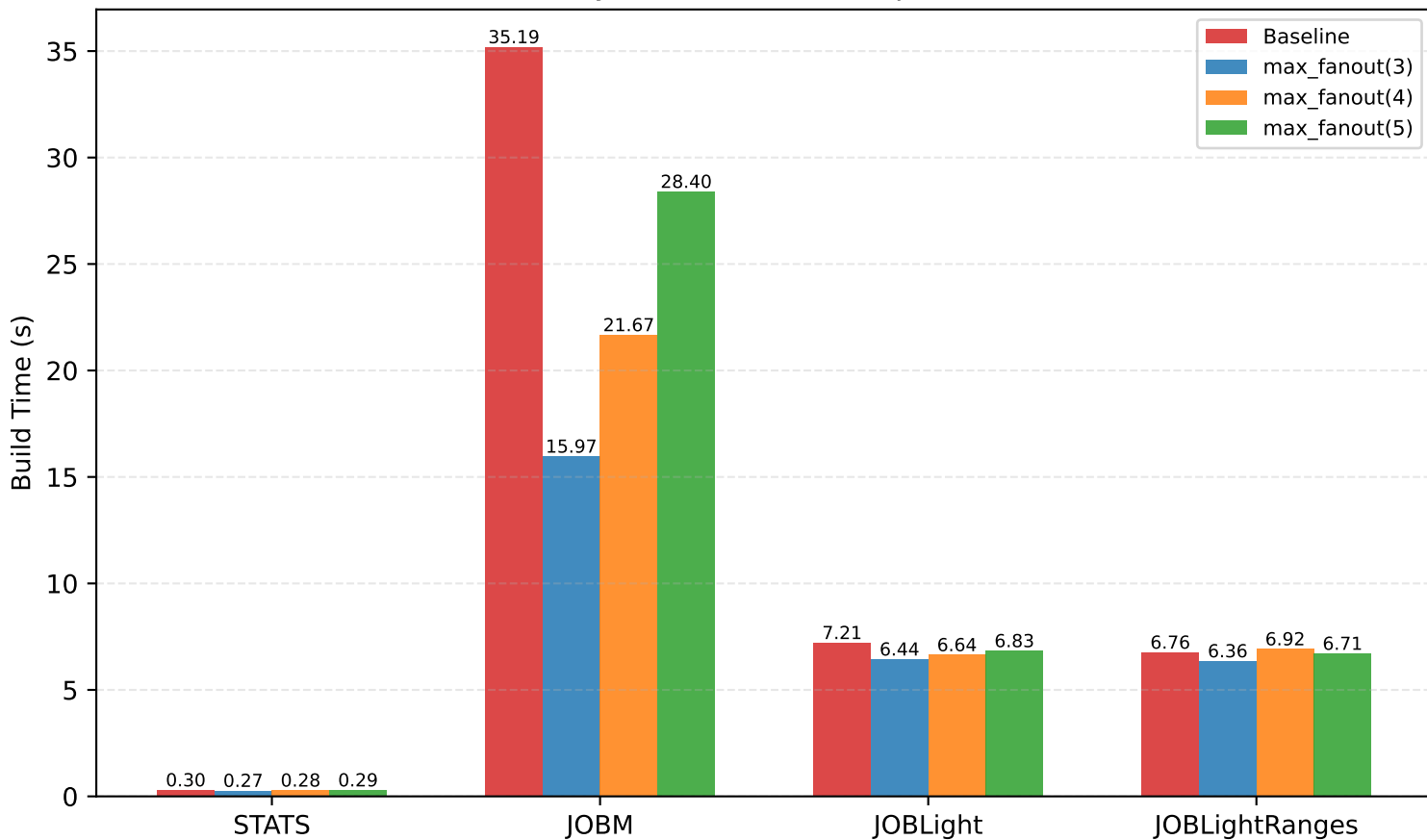
Build Time by Benchmark and SplitStar Variant
