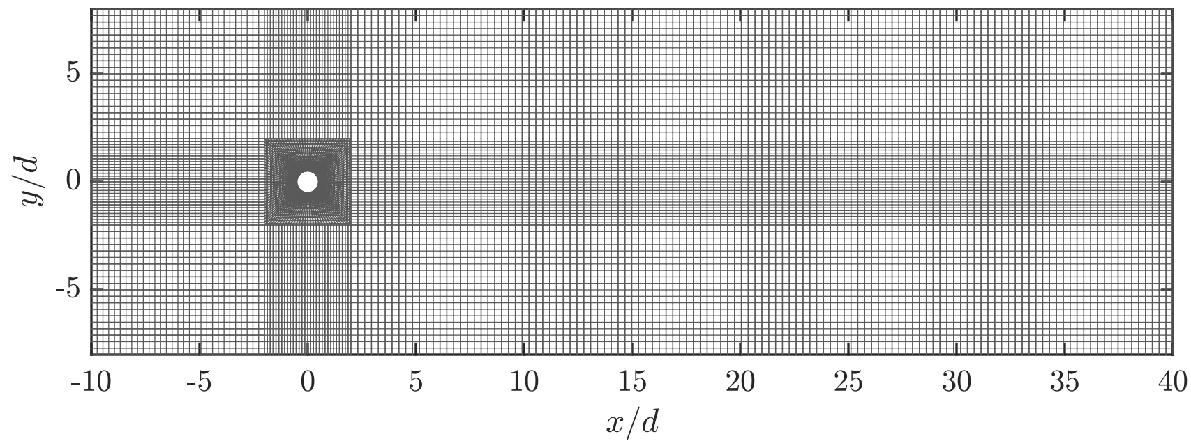
Computational Mesh
