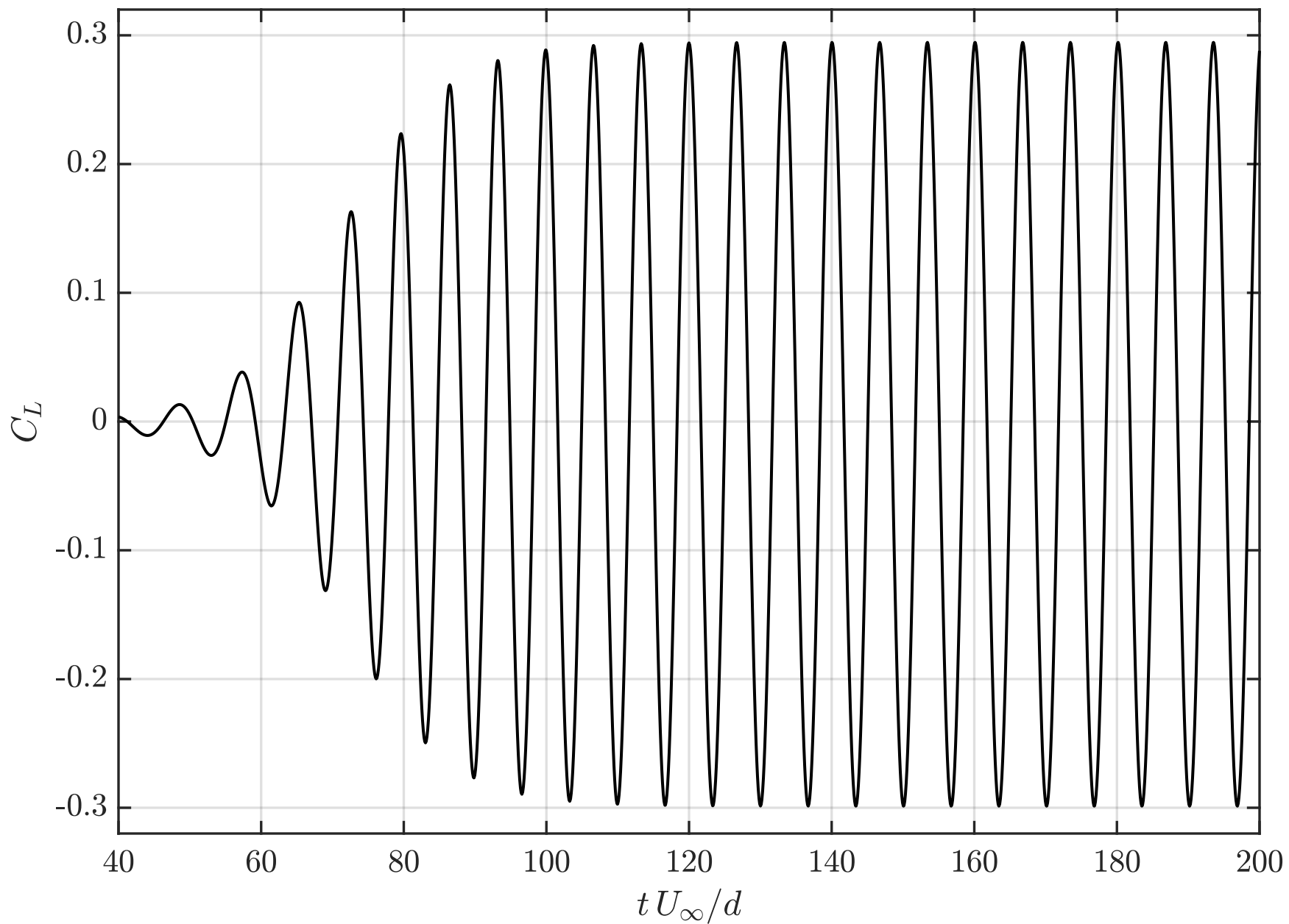
Lift Coefficient History — Closeup
