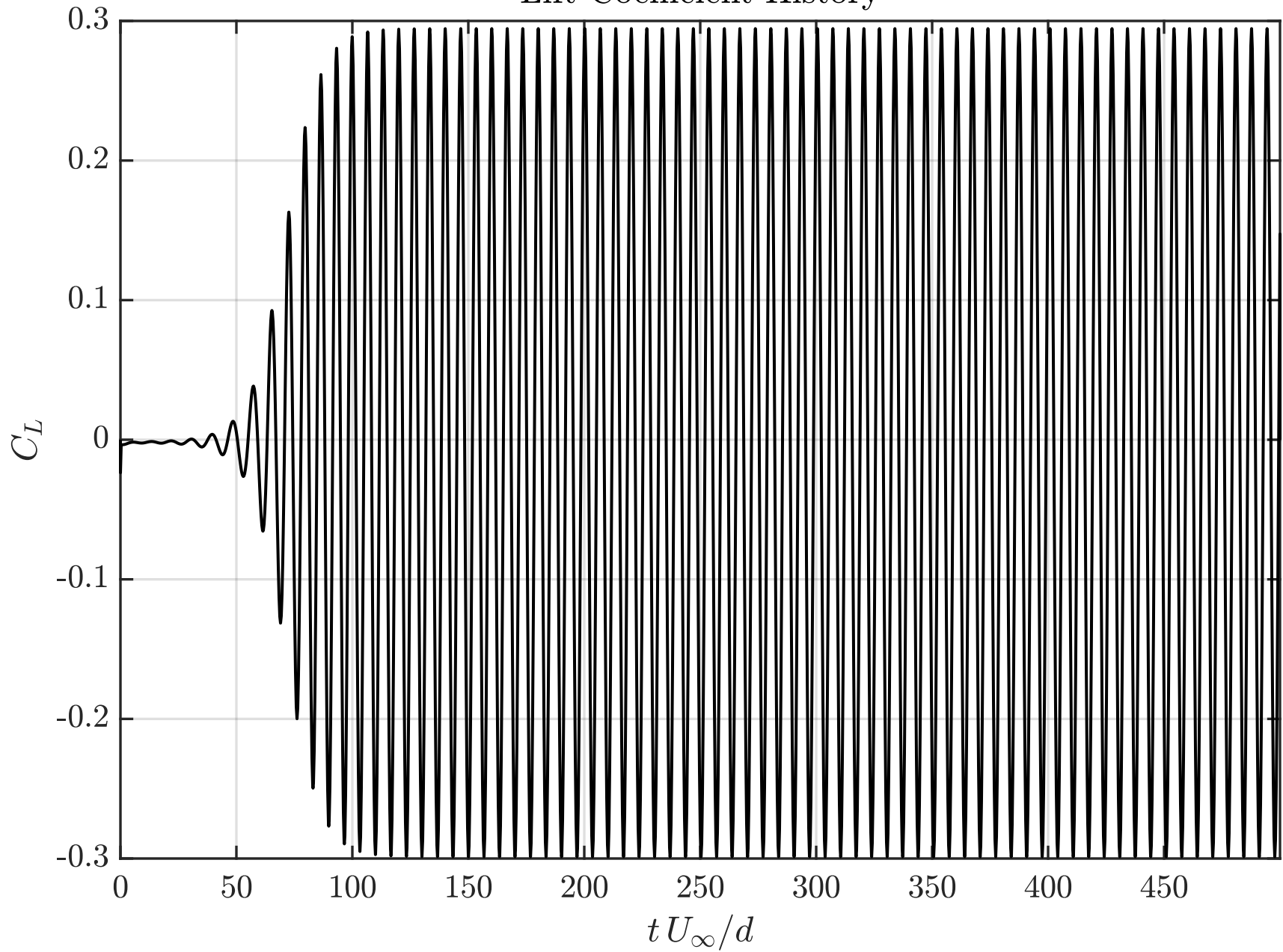
Lift Coefficient History
