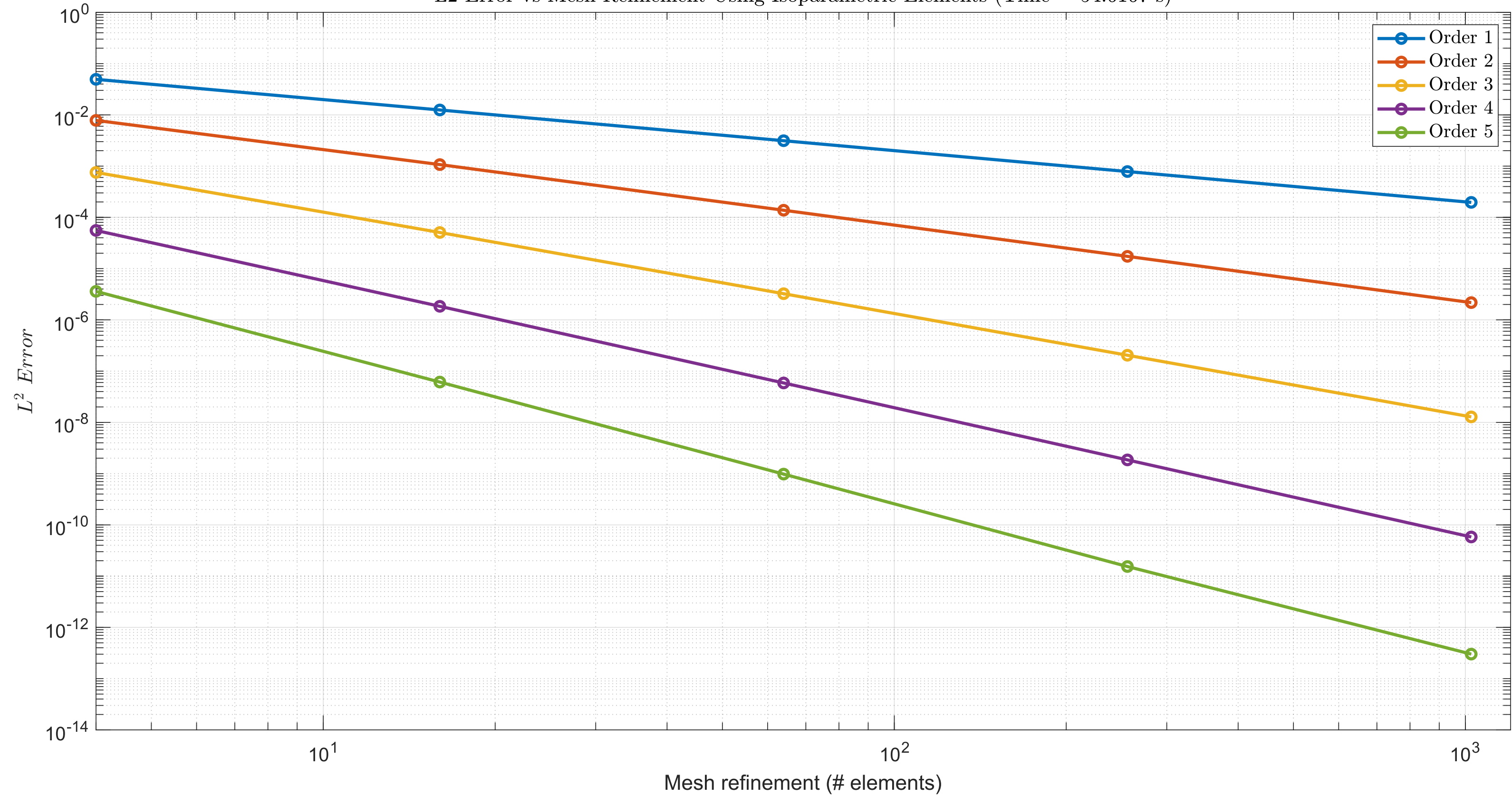
L2 Error vs Mesh Refinement Using Isoparametric Elements (Time = 54.6167 s)
