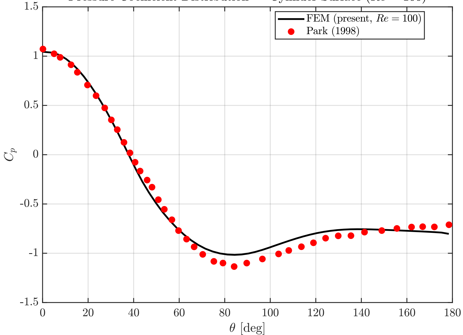
Pressure Coefficient Distribution — Cylinder Surface ( Re = 100 )
