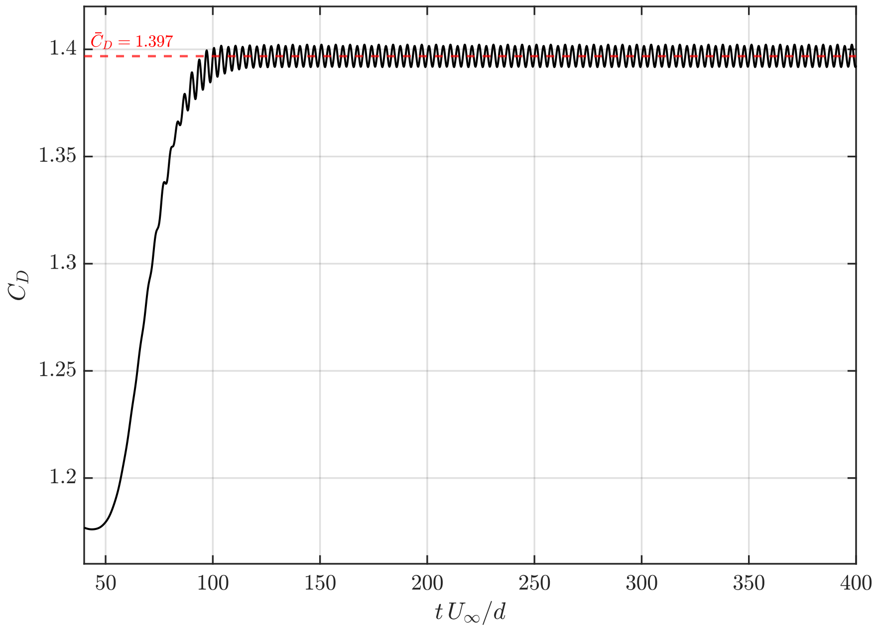
Drag Coefficient History
