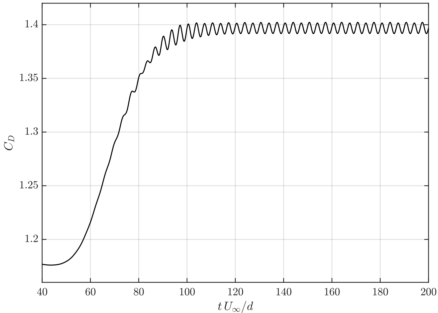
Drag Coefficient History — Closeup
