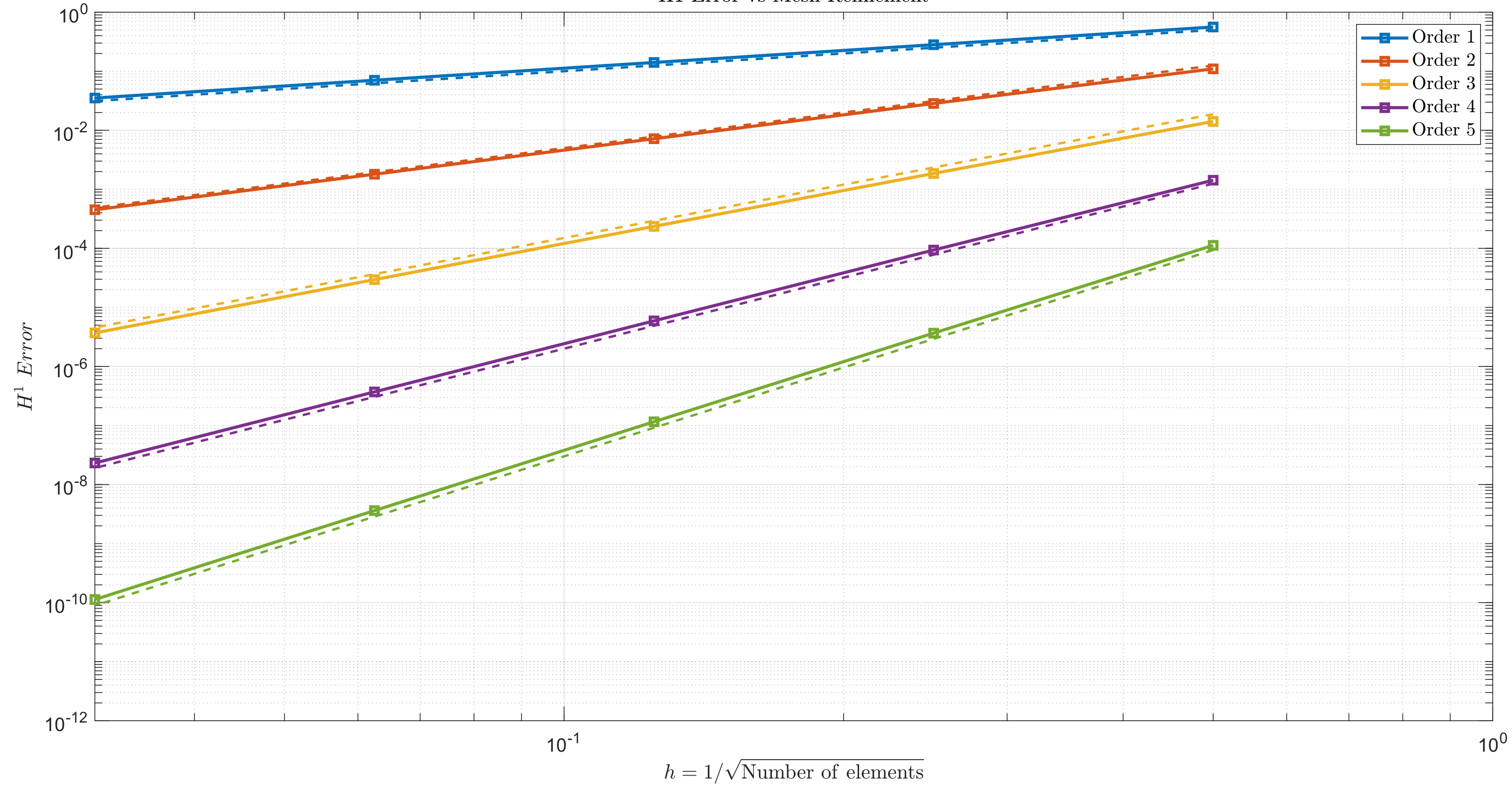
H1 Error vs Mesh Refinement
