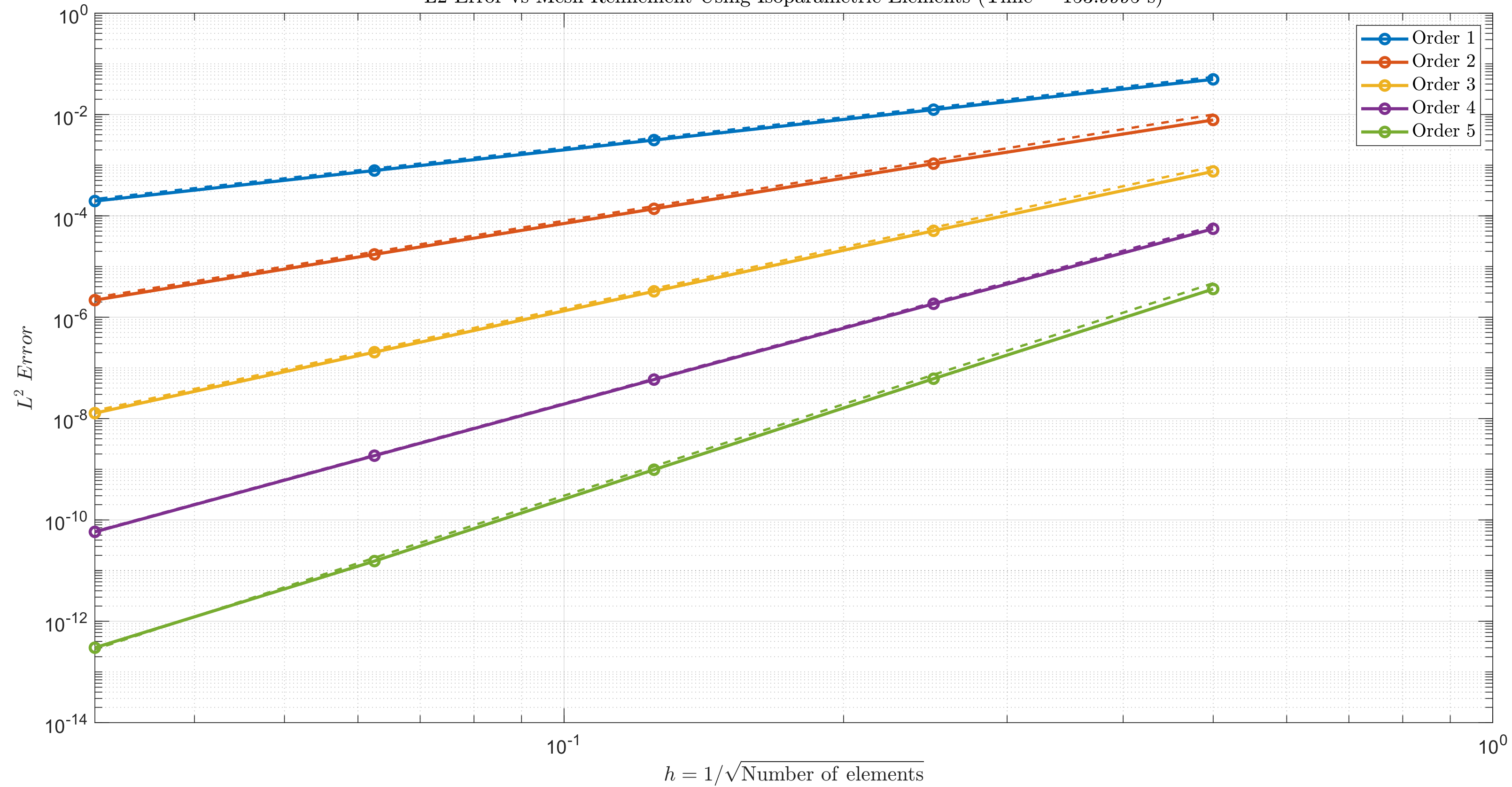
L2 Error vs Mesh Refinement Using Isoparametric Elements (Time = 153.9995 s)
