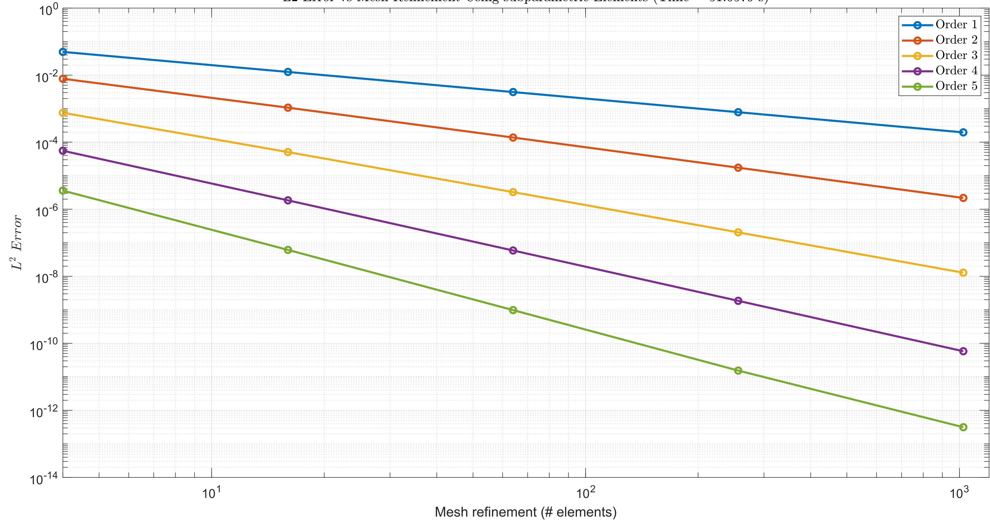
L2 Error vs Mesh Refinement Using subparametric Elements (Time = 51.6579 s)
