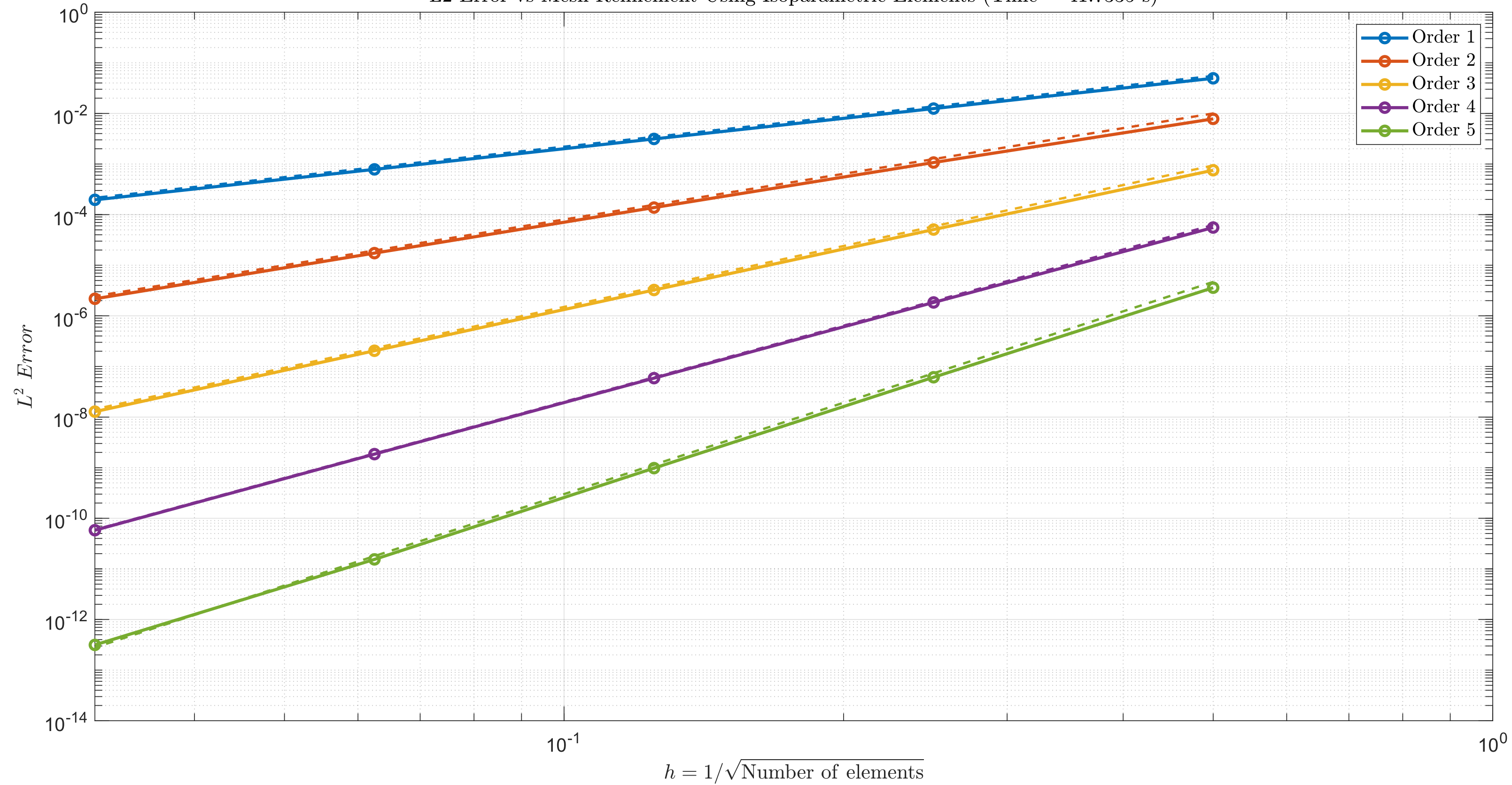
L2 Error vs Mesh Refinement Using Isoparametric Elements (Time = 41.7335 s)
