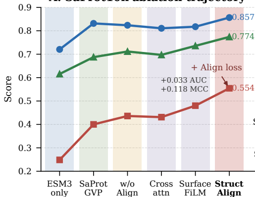
A. SaProt10k ablation trajectory
