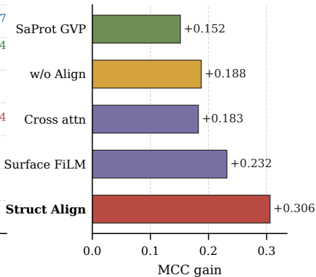
B. MCC gain over ESM3-only
