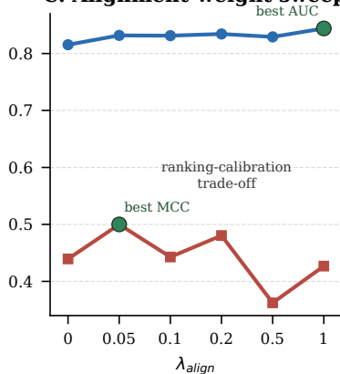
C. Alignment-weight sweep
